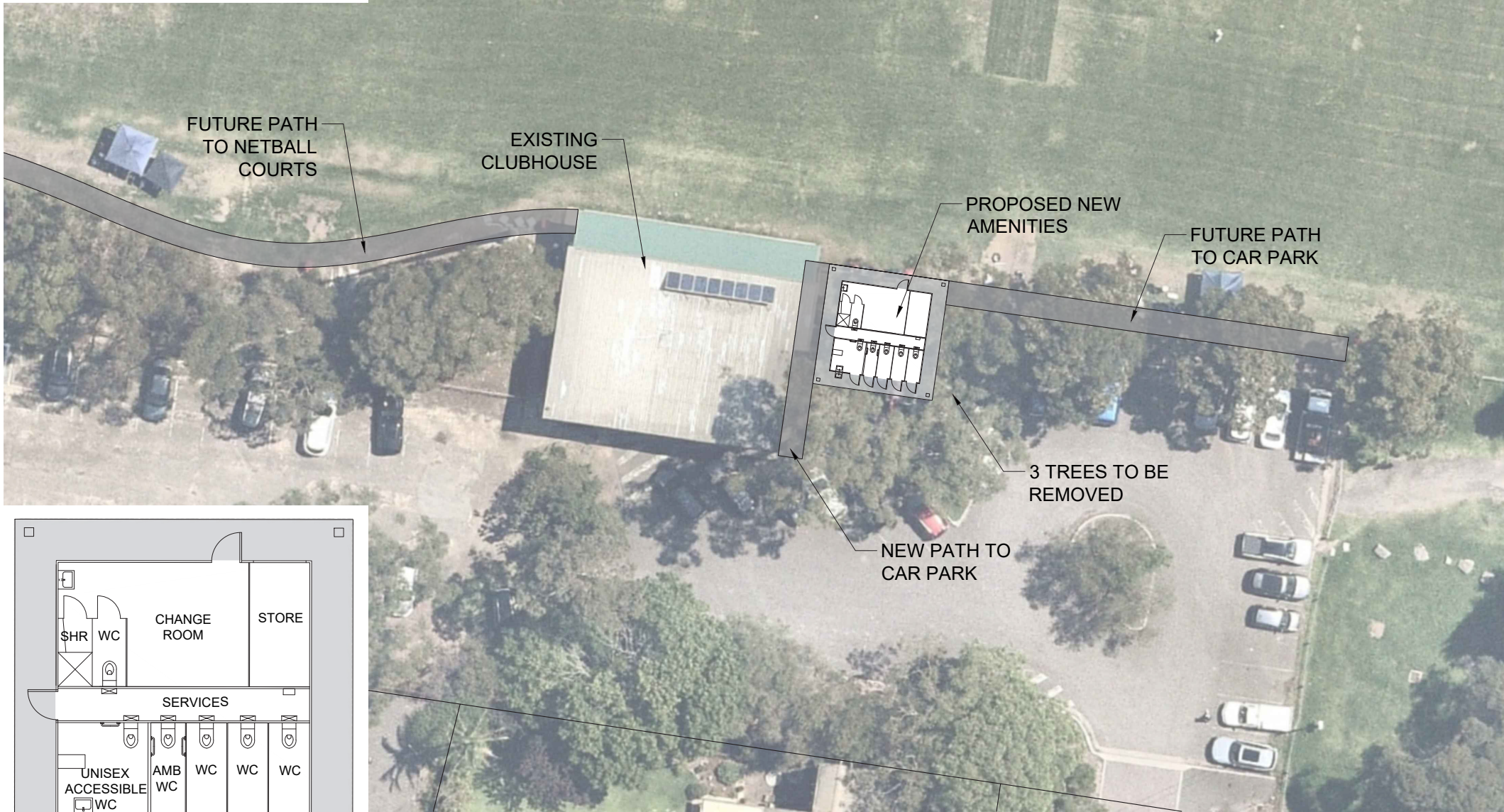
CONTEXT PLAN
